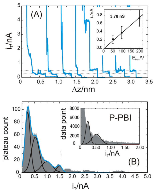
Figure 4. (A) Typical current–distance ( i_T – \Delta z ) retraction curves for P-PBI molecules immobilized on Au(111)-(1 × 1) in 50 mM LiClO 4 , pH ~ 12, at E_{\text{bias}} = 0.05 V; E_S = -0.12 V (versus SCE). The inset shows a linear dependence of the conductance current (obtained from statistical analysis) on the bias voltages. (B) Plateau-counting conductance histograms constructed from type III current–distance curves of P-PBI, 250 type III out of 2500 recorded traces; 5 pA bin size. The inset shows the corresponding data-point conductance histograms constructed from the same sets of single traces. The peak positions were determined by Gaussian fits.
